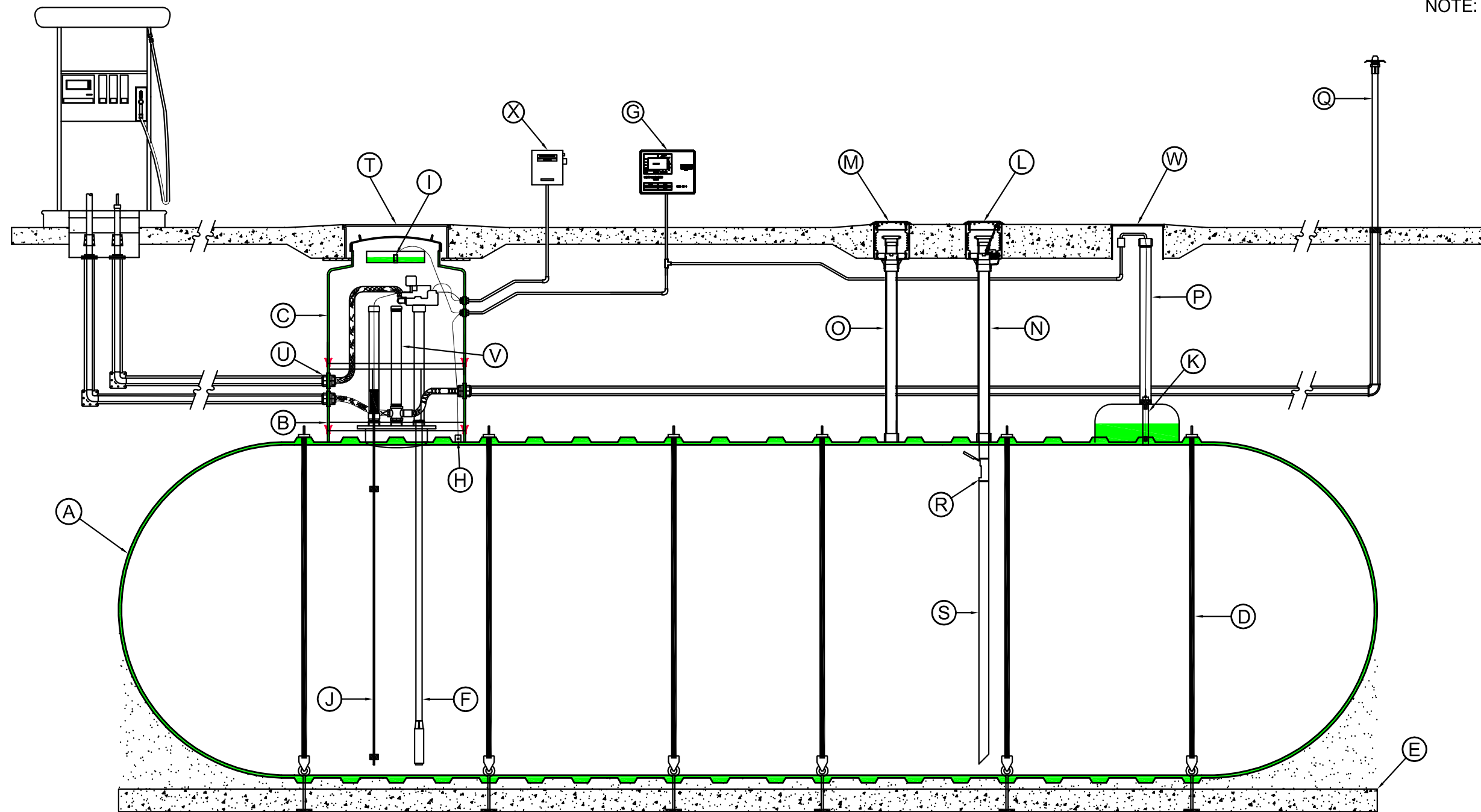
HYDROGUARD® SYSTEM TYPICAL ILLUSTRATION DRAWING SINGLE-SUMP SYSTEM - (10') 20,000 GALLON DOUBLE-WALL TANK w/ DOUBLE-WALL TURBINE SUMP
