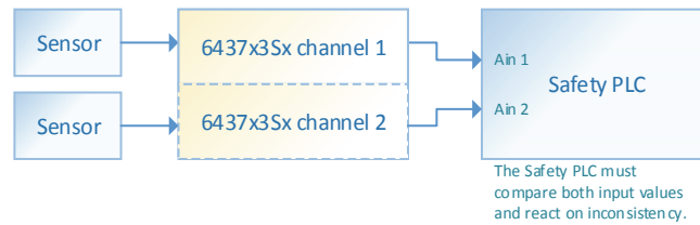
Figure 6 6437 Dual channel 1oo2 operation
