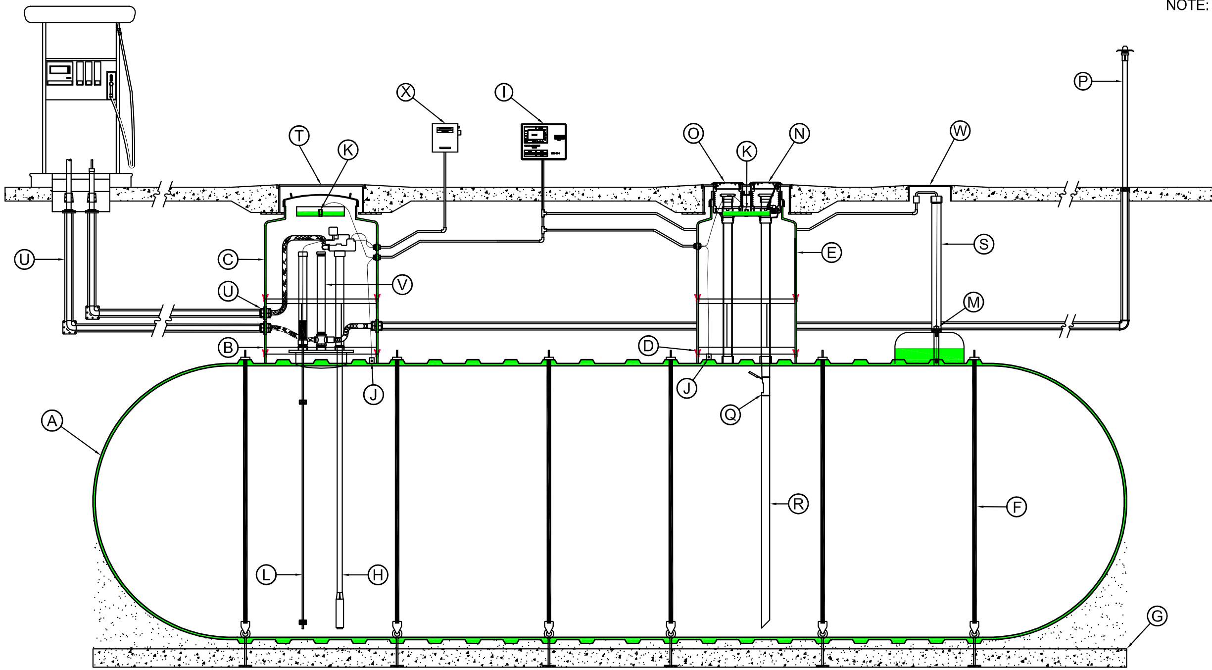
HYDROGUARD® SYSTEM TYPICAL ILLUSTRATION DRAWING MULTI-SUMP SYSTEM - (10') 20,000 GALLON DOUBLE-WALL TANK w/ DOUBLE-WALL TURBINE AND FILL/VAPOR SUMP
