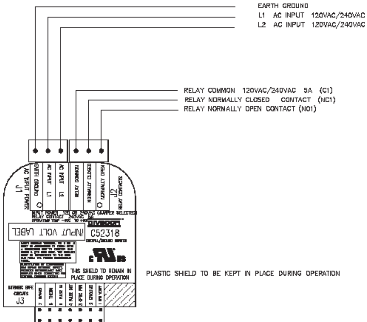
FIGURE 3 - Power Wiring
