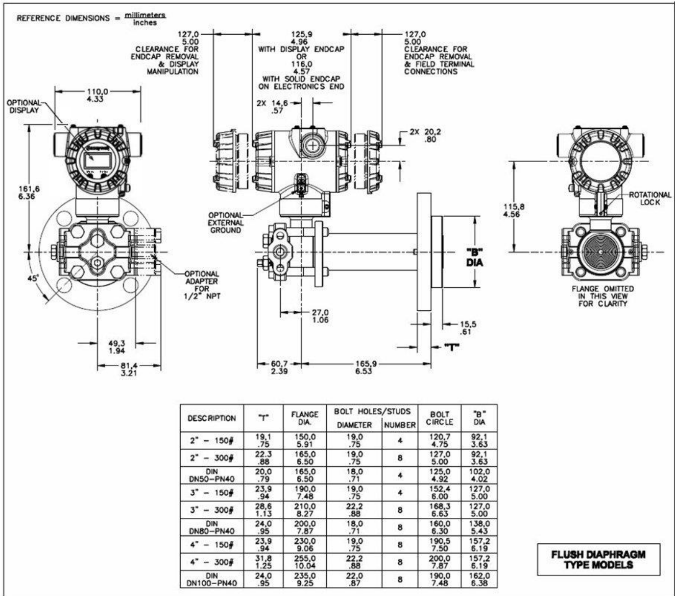
Figure 4 – Typical mounting dimensions for flush diaphragm type models STF725 and STF735.
