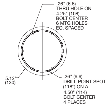
Holder Mounting SP-FU/MHCF
