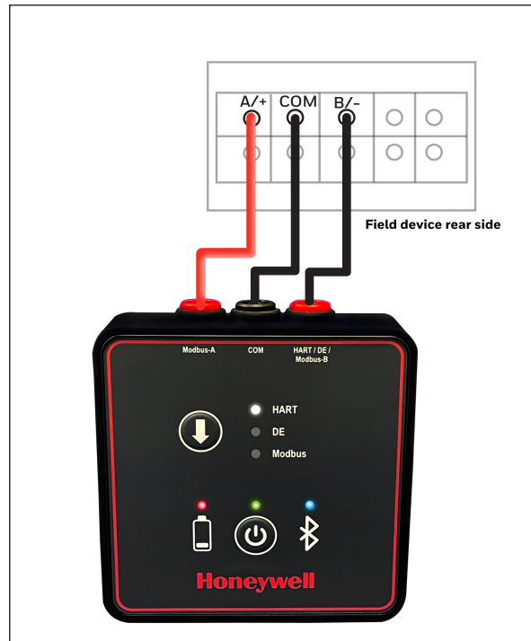
Figure 3-2: Connect to the Modbus field devices
