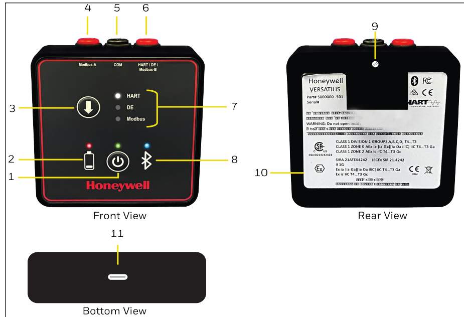
Figure 2-1: Modem overview
