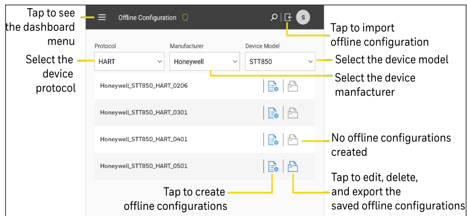
Figure 4-18: Offline configuration
