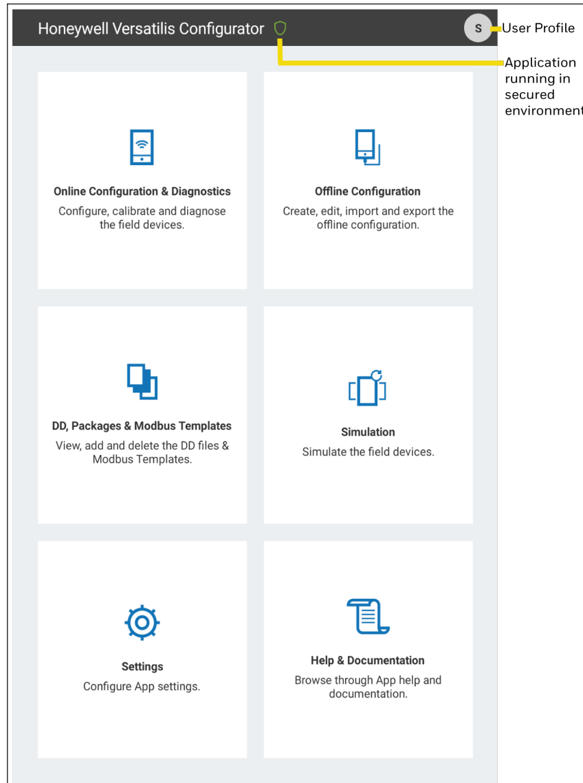
Figure 4-1: Dashboard screen
