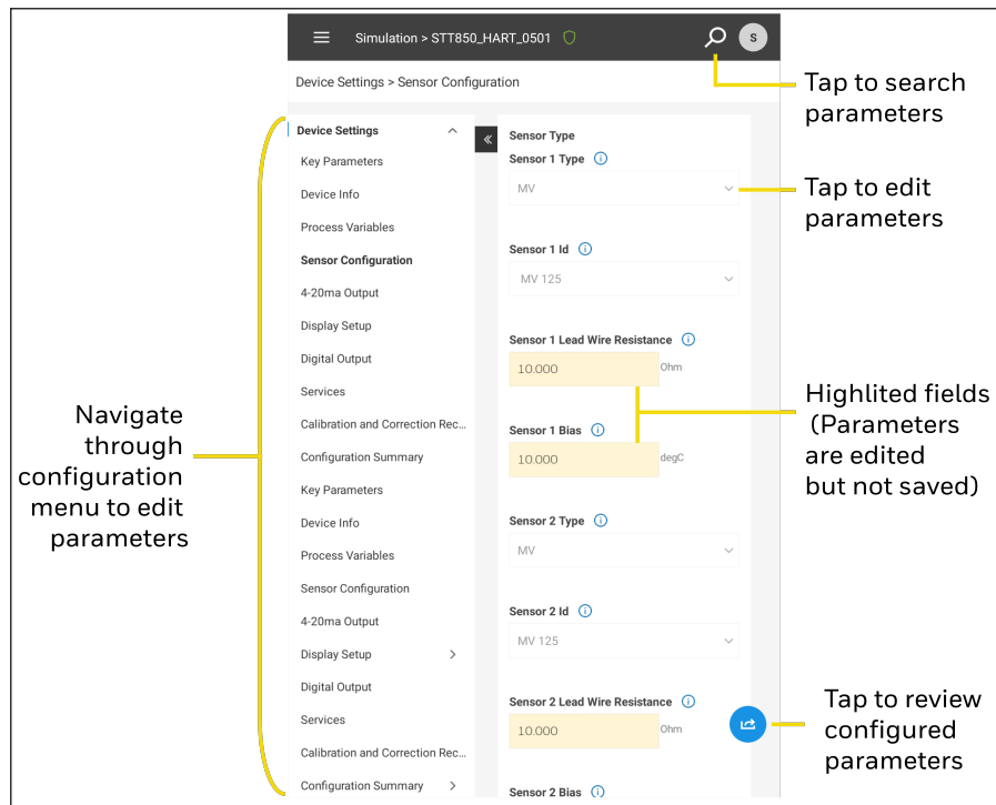
Figure 4-30: Device simulation
