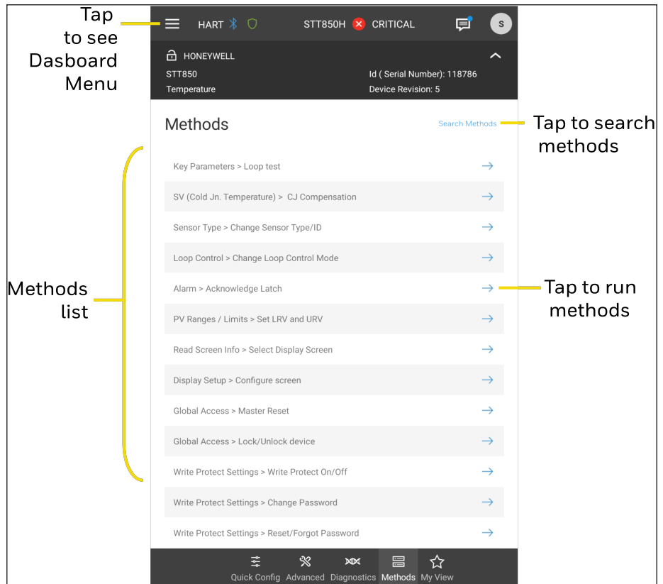
Figure 4-14: Methods screen
