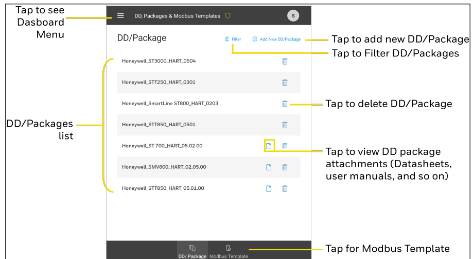
Figure 4-21: Manage DD/Packages
