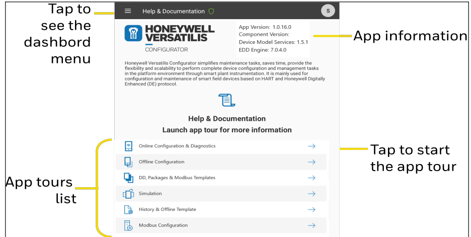
Figure 4-33: Help & documentation
