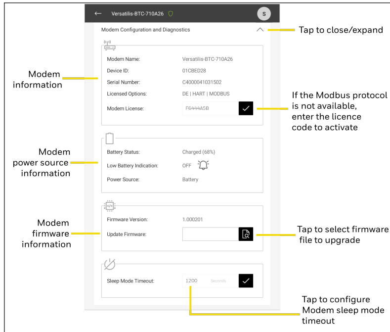
Figure 4-6: Modem using batteries
