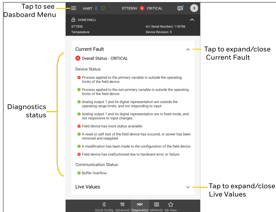
Figure 4-13: Diagnostics screen
