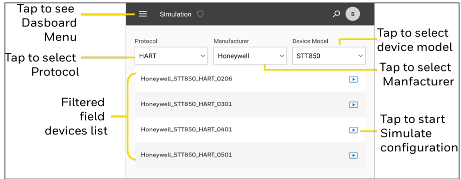
Figure 4-29: Simulation
