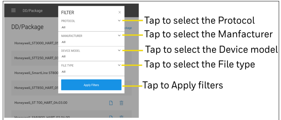
Figure 4-22: DD/Package filter
