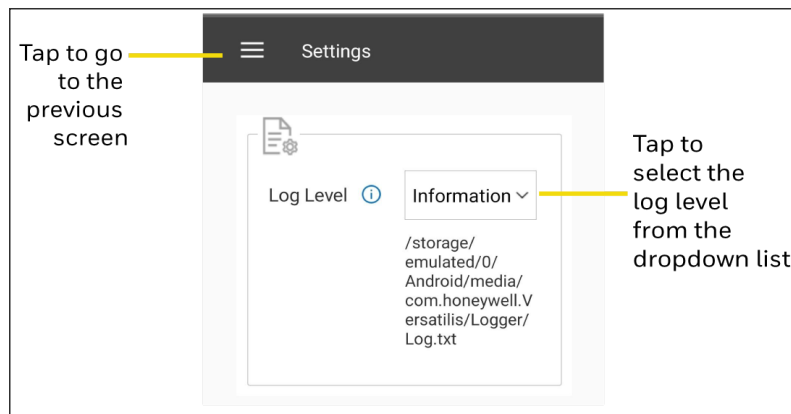
Figure 4-32: Settings
