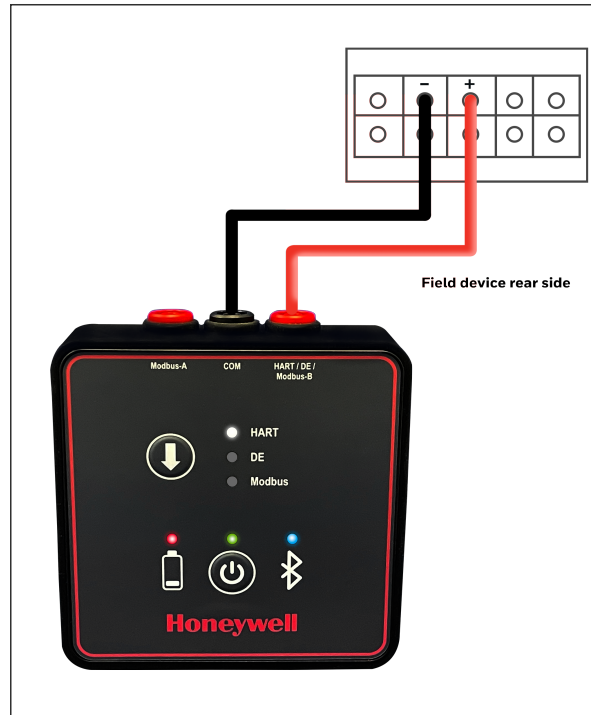
Figure 3-1: Connect to the HART/DE field devices
