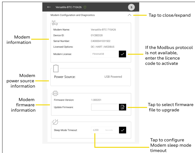
Figure 4-7: Modem using USB power
