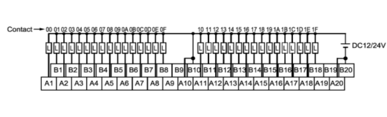
MLE-TN32A Output Wiring Diagram (TG7-1H40S)
